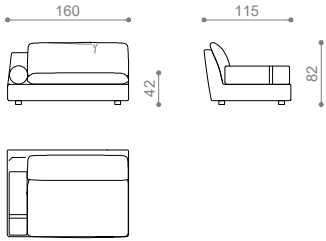
COD. N167004 SX/DX terminale | end element
