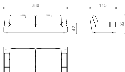
COD. N167002 divano | sofa
